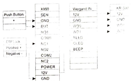
X-990 with KR 500 and EM Lock Connection
