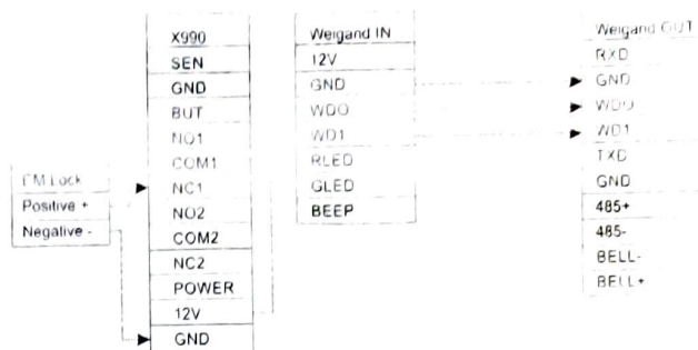
X-990 Master Device
