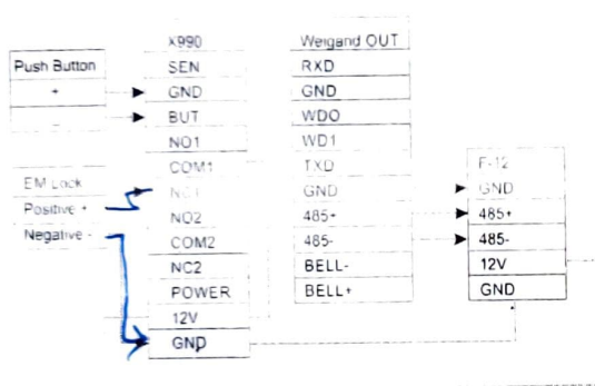
X-990 with F-12 and EM Lock connection
